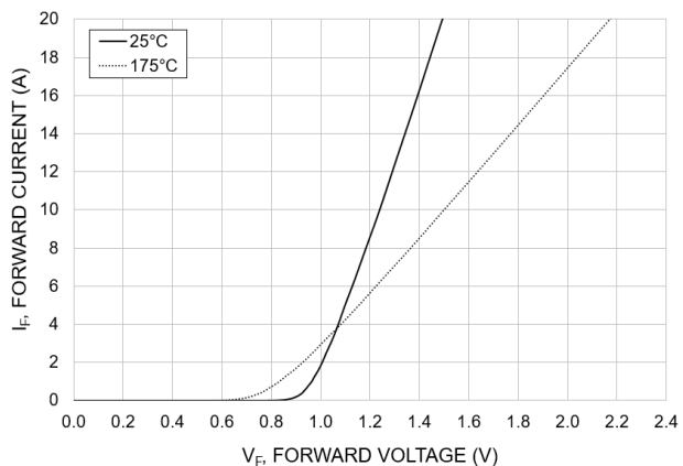
Figure 5. Boost Diode Forward Characteristics
