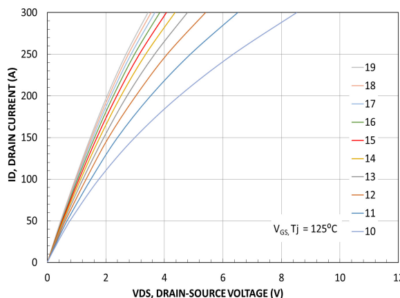
Figure 3. MOSFET Typical Output Characteristics
