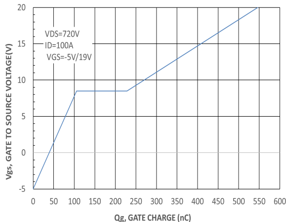
Figure 7. Gate-to-Source Voltage vs. Total Charge
