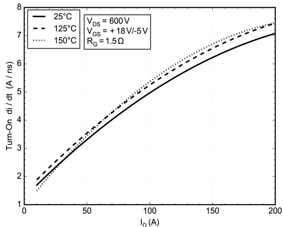
Figure 21. di/dt ON vs I_D
