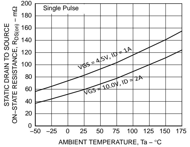
Figure 5. R_{DS(on)} - T_a
