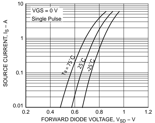
Figure 7. I_S - V_{SD}
