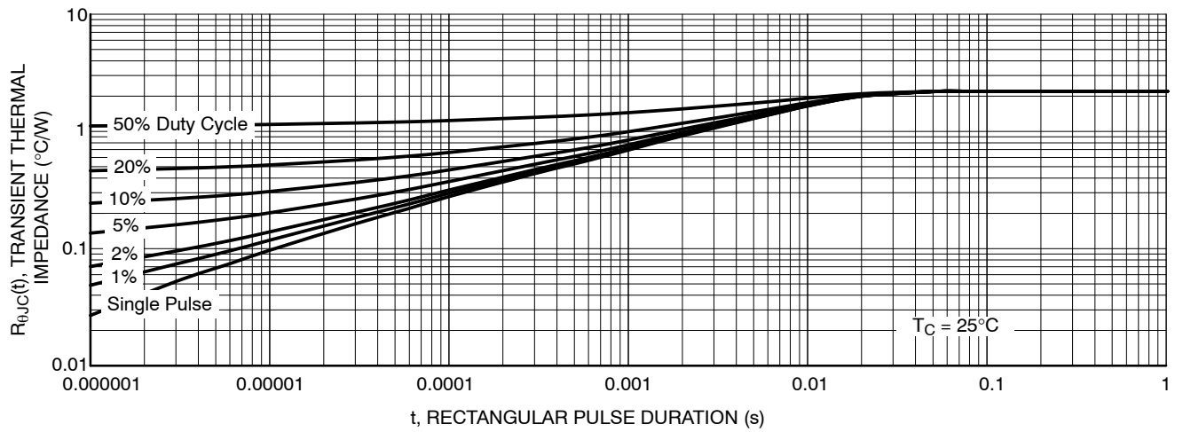
Figure 14. Thermal Response
