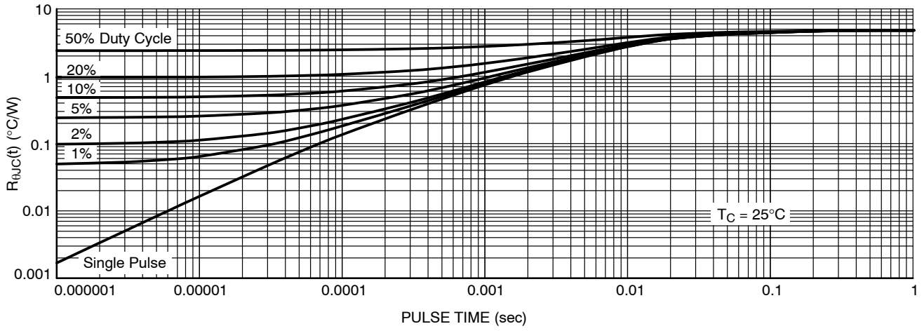
Figure 14. Thermal Characteristics
