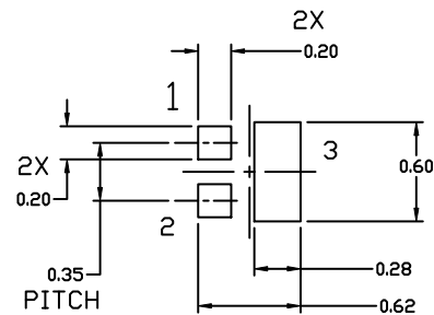
RECOMMENDED MOUNTING FOOTPRINT
