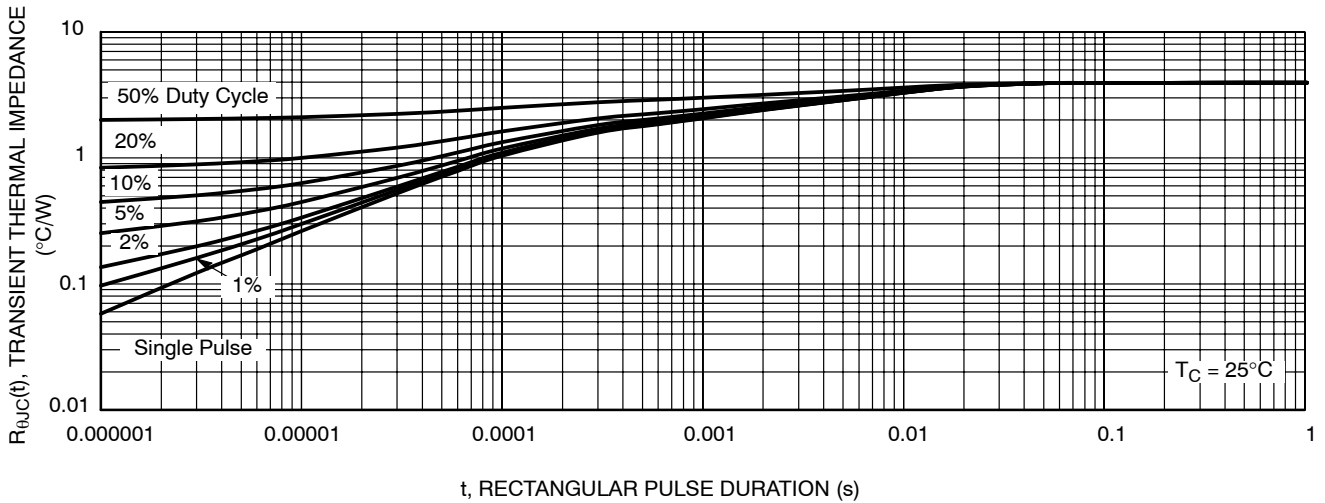
Figure 14. Thermal Response
