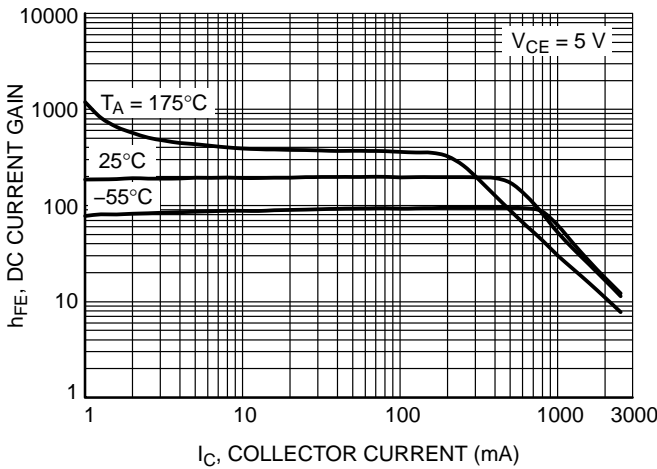
Figure 4. hFE - IC
