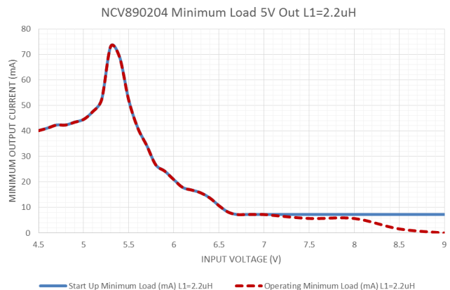
Typical Minimum Load 5 V Out, L1 = 2.2 µH
