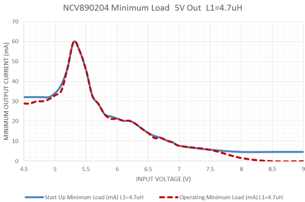
Typical Minimum Load 5 V Out, L1 = 4.7 µH
