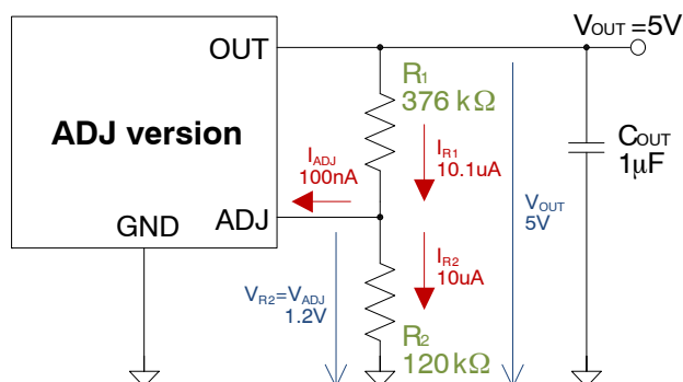
Figure 54. ADJ Output Voltage Schematic – Example 2
