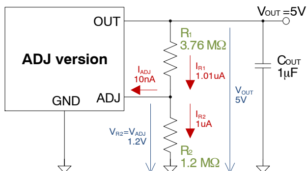
Figure 53. ADJ Output Voltage Schematic – Example 1
