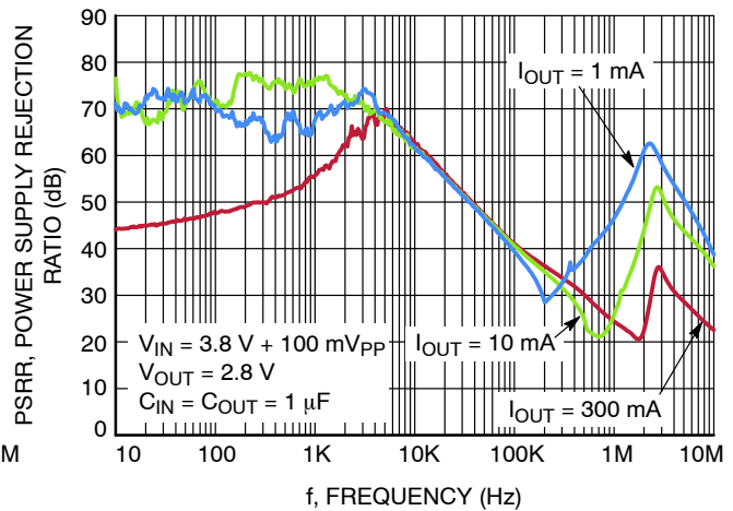
Figure 18. PSRR vs. Frequency, V OUT = 2.8 V
