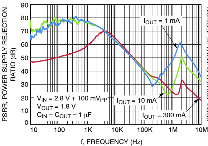
Figure 17. PSRR vs. Frequency, V OUT = 1.8 V
