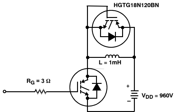
Figure 18. Inductive Switching Test Circuits
