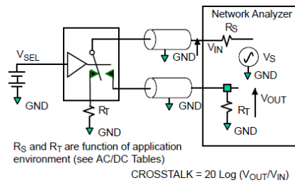
Figure 15. Adjacent Channel Crosstalk
