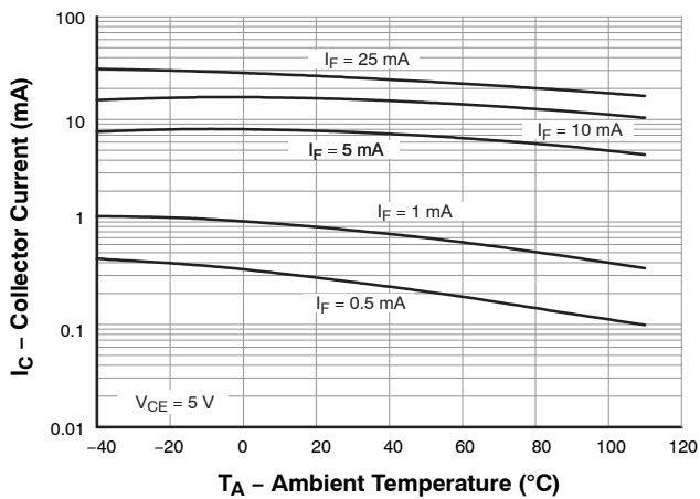
Figure 5. Collector Current vs. Ambient Temperature (FODM121/2701/2705)
