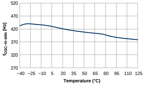
Figure 11. Minimum Frequency at No Load ( f_{OSC-N-MIN} ) vs. Temperature
