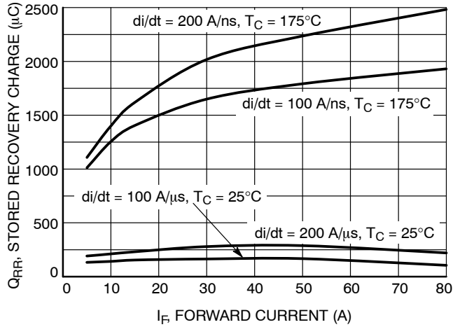
Figure 20. Stored Charge
