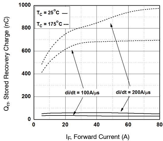
Figure 20. Stored Charge
