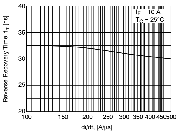
Figure 6. Typical Reverse Recovery Time vs. di_F/dt
