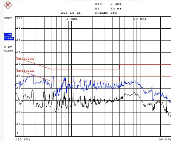
Date: 29.AUG.2011 17:20:36 Figure 35. Conduction Line at 230V AC 50% Load
