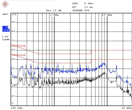
Date: 29.AUG.2011 17:14:16 Figure 36. Conduction Neutral at 115V AC 50% Load
