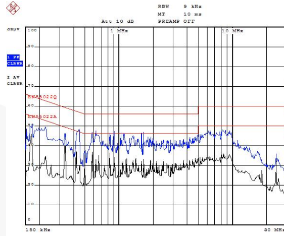
Date: 29.AUG.2011 16:04:59 Figure 33. Conduction Neutral at 230V AC 75% Load
