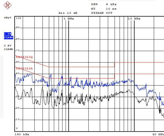
Date: 29.AUG.2011 17:22:33 Figure 37. Conduction Neutral at 230V AC 50% Load
