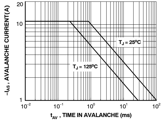
Figure 10. Unclamped Inductive Switching Capability
