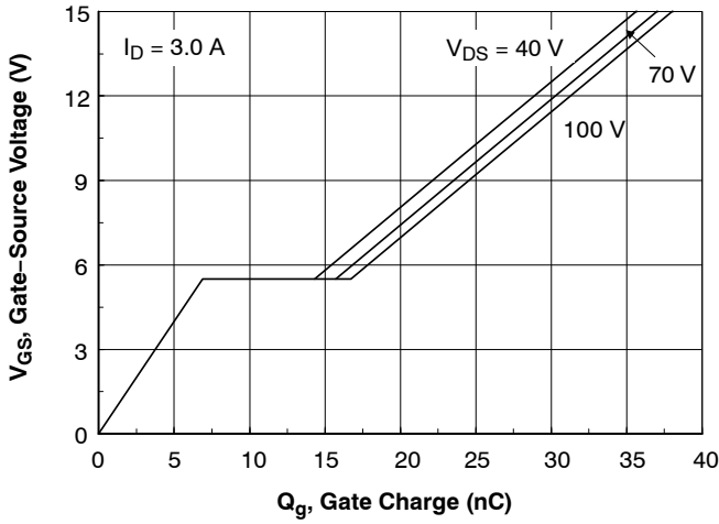
Figure 7. Gate-Charge Characteristics
