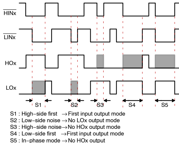
Figure 40. Interlock Function
