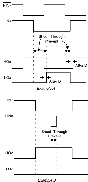
Figure 39. Shoot-Through Protection
