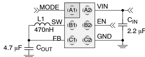
Figure 1. Typical Application
