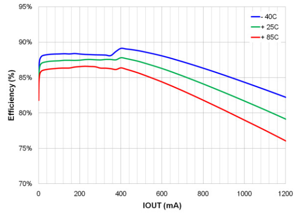
Figure 5. Efficiency vs. Load Current and Temperature
