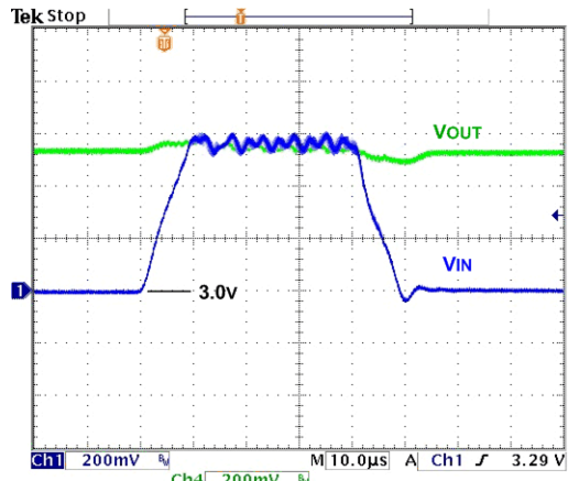
Figure 25. Line Transient, 3.0–3.6 V_{IN} , 10 μs Edge, 1,000 mA Load, V_{OUT} = 3.5\text{ V}
