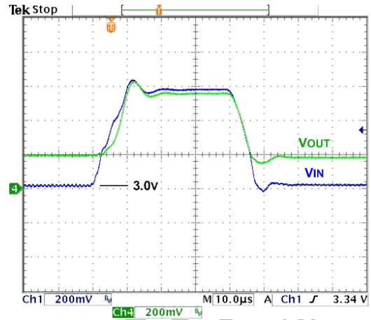
Figure 24. Line Transient, 3.0–3.6 V_{IN} , 10 μs Edge, 500 mA Load, V_{OUT} = 3.15\text{ V}
