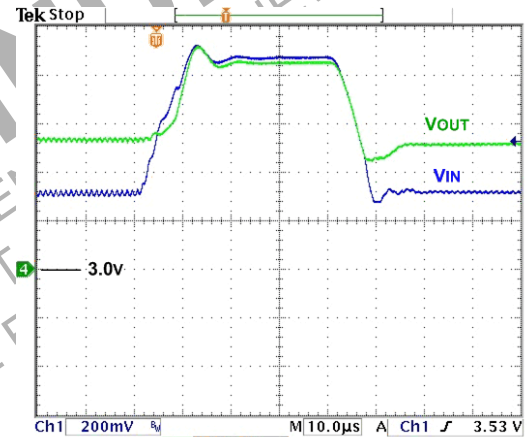
Figure 26. Line Transient, 3.3–3.9 V_{IN} , 10 μs Edge, 500 mA load, V_{OUT} = 3.5\text{ V}
