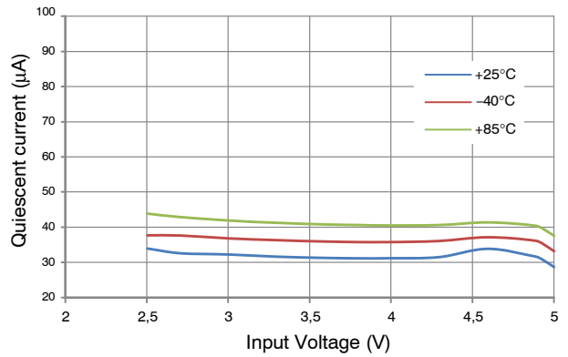
Figure 8. Quiescent Current
