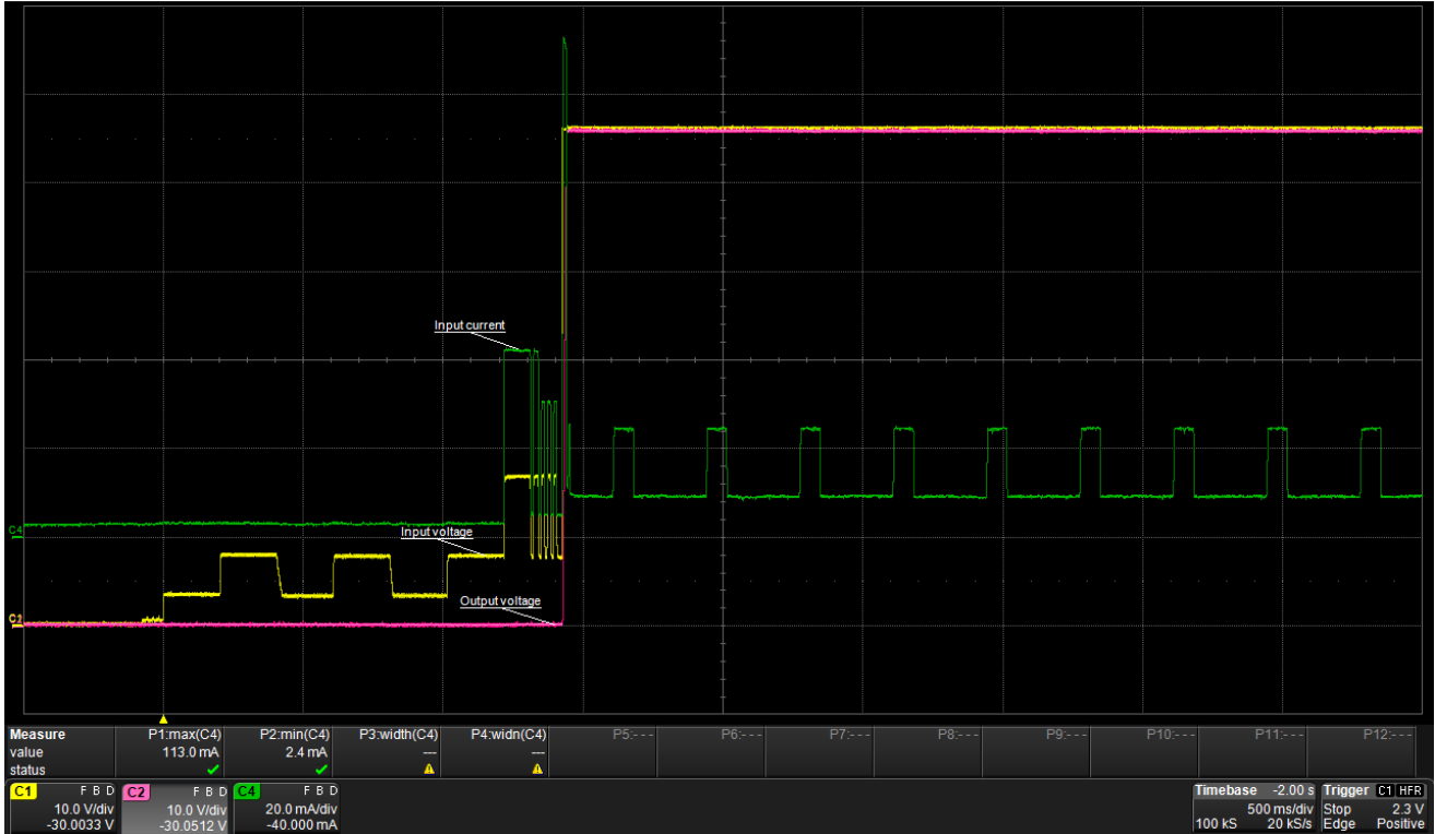
Figure 17. No Load Start-up, MPS Circuit Turned ON
