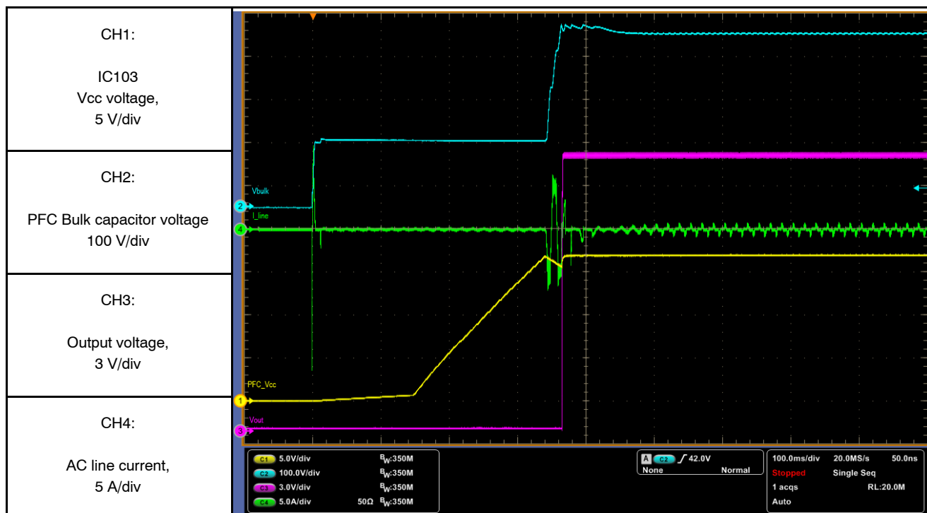
Figure 75. Start-up Sequence into Constant Current Load 1 A / \approx 19 W
