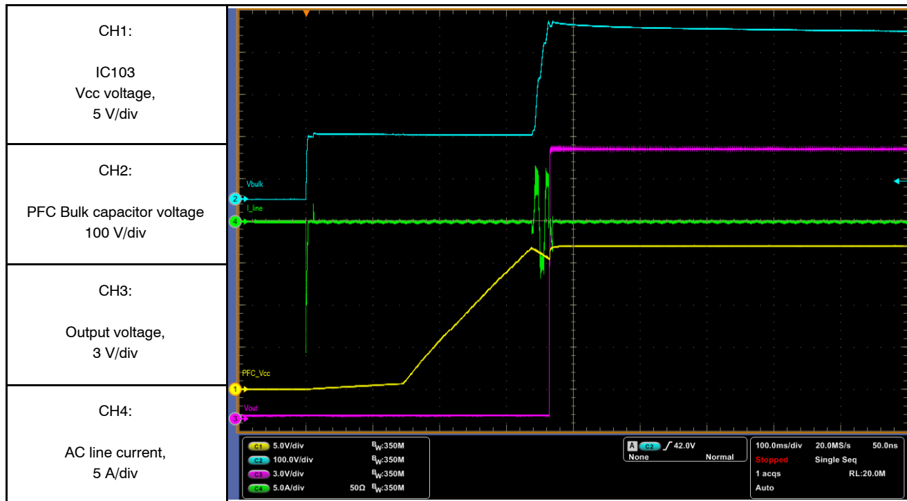
Figure 74. Start-up Sequence without Loading (0 A)
