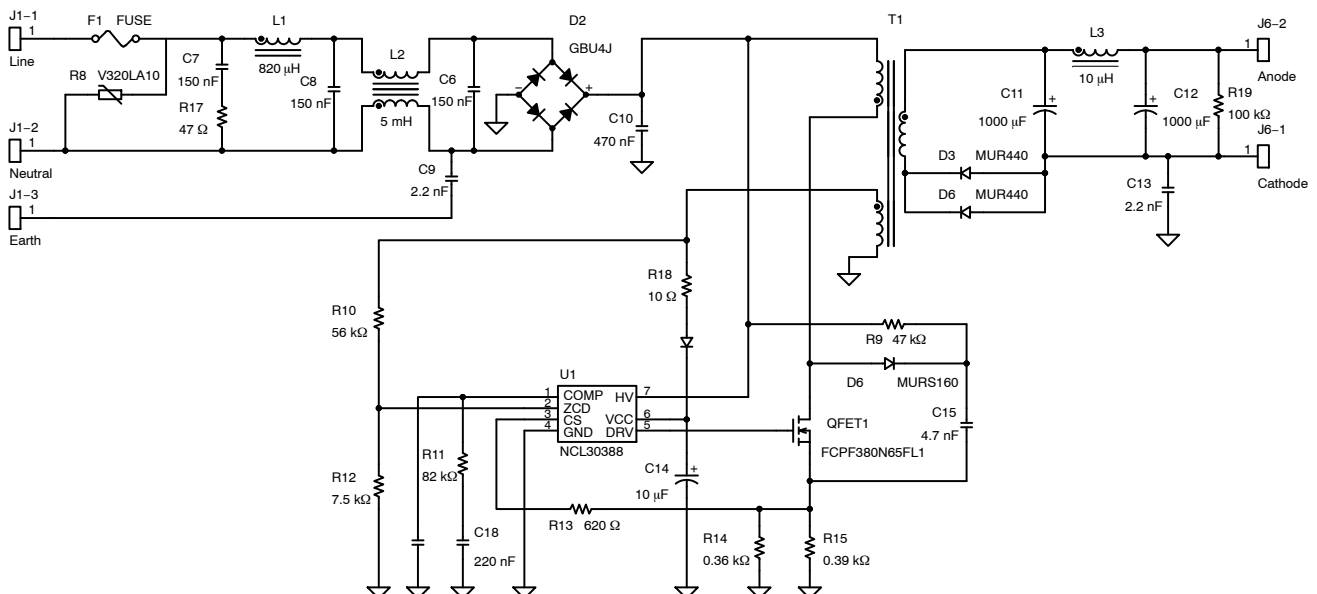
Figure 3. Schematic
