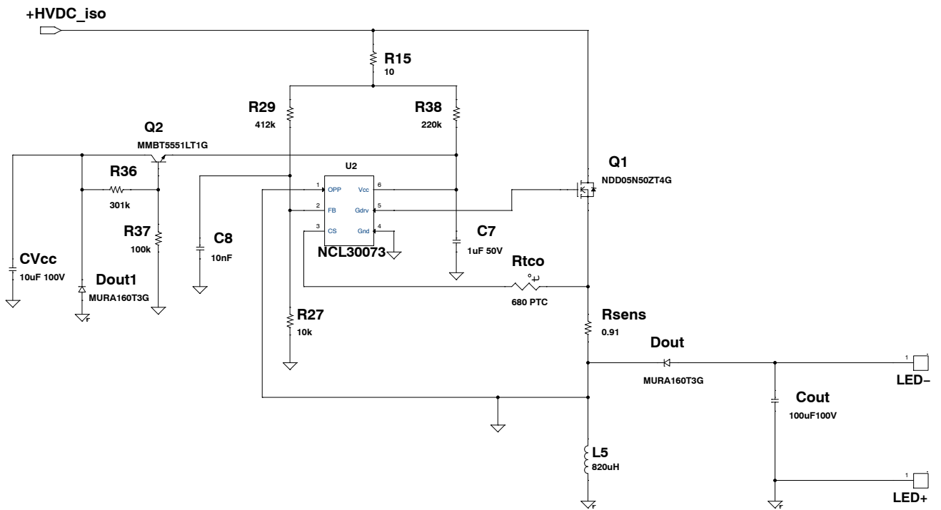
Figure 4. Main Circuit
