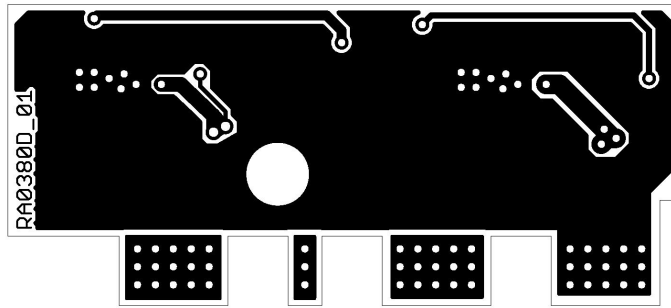
Figure 7. SR Daughtercard Board Bottom Layer
