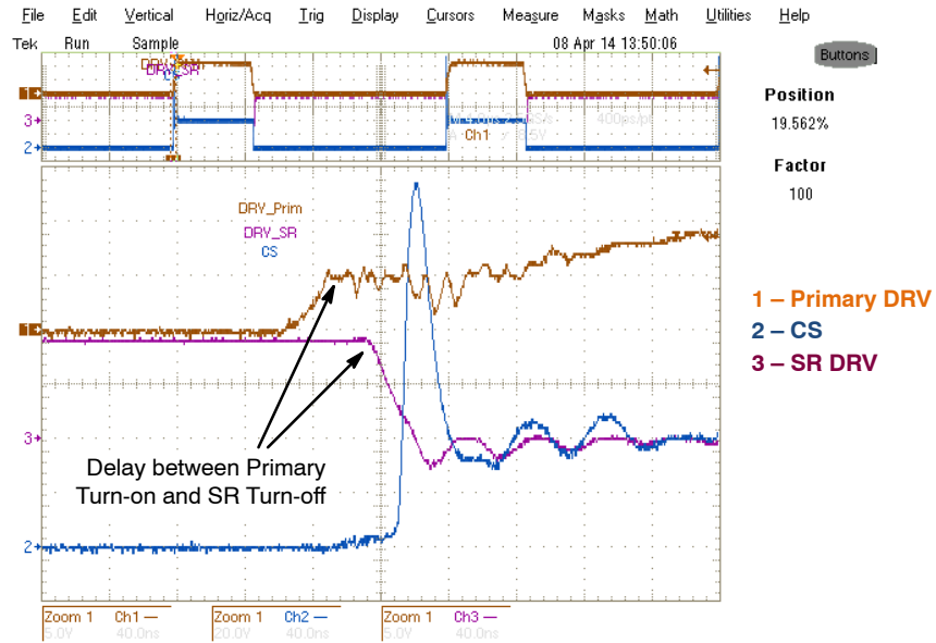
Figure 18. V_{IN} = 180 \text{ V}_{AC} , I_{OUT} = 5.8 \text{ A} , SR Transistor is Turned-off after Primary Side is Turned-on and Shot through Condition Occurs
