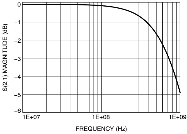
Figure 9. Insertion Loss
