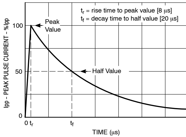
Figure 11. 8 X 20 \mu s Pulse Waveform
