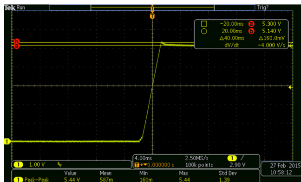
Figure 25. 115 Vac and No Load
