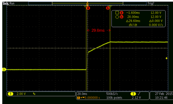
Figure 23. 115 Vac and 2 A CC Load
