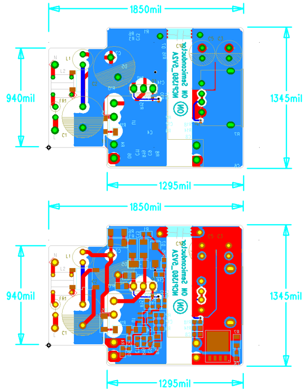
Figure 1. PCB Layout
