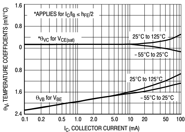
Figure 9. Temperature Coefficients
