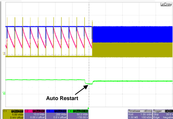
Figure 28. V_{IN} = 300 V_{AC} / 50 Hz , [LED Restore]
