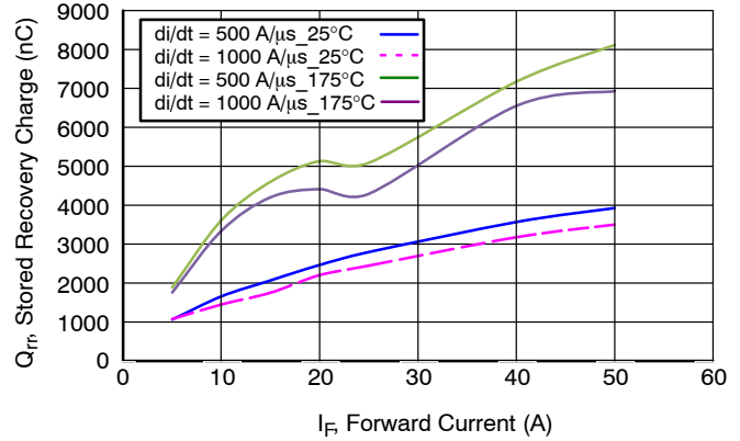
Figure 18. Stored Charge
