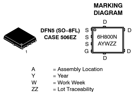
N-CHANNEL MOSFET
