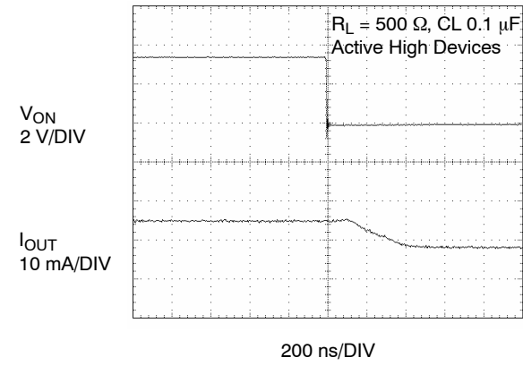
Figure 19. T_{OFF} Response
