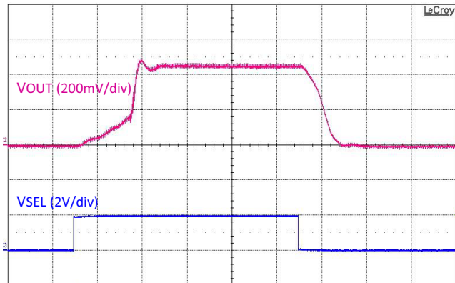
Figure 21. V_{SEL} Step, V_{IN} = 3\text{ V} , V_{OUT} = 3.15 \leftrightarrow 3.6\text{ V} , I_{OUT} = 500\text{ mA}
