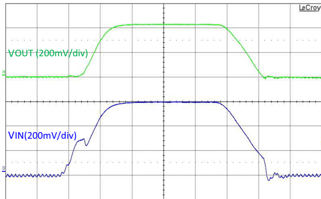
Figure 19. Line Transient, V_{IN} = 3.0\text{ V} \leftrightarrow 3.6\text{ V} , 10\ \mu\text{s} Edge, I_{OUT} = 500\text{ mA} , V_{OUT} = 3.15\text{ V}
