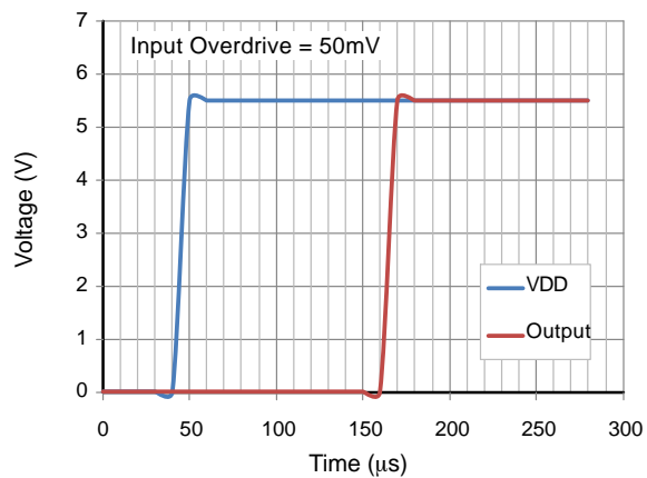
Figure 13. Power-Up Delay
