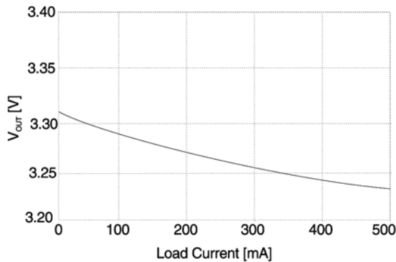
Figure 2. Load Regulation
