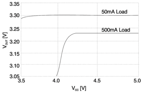
Figure 1. Dropout Characteristics
