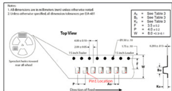
New Die orientation (Pin 1 bottom right)
