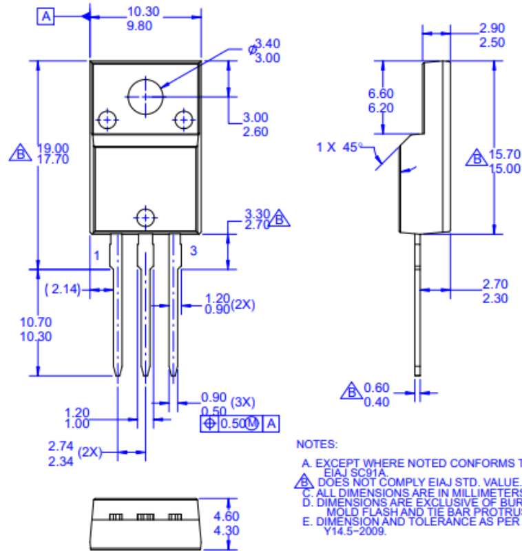
TO-220 FULLPACK, 3-LEAD CASE 221BN ISSUE O
