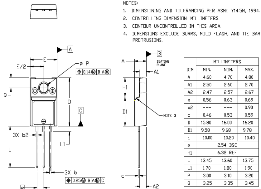
TO-220 FULLPACK, 3-LEAD CASE 221BN ISSUE O
