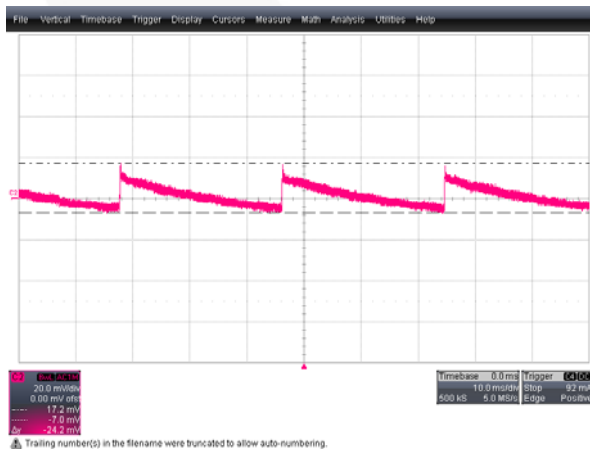
Figure 24. V_{O\_RIPPLE} = 24.2\text{mV} , Output with 90\text{V}_{AC} and No-Load Condition, CH2: V_O (20mV/div), Time: 10ms/div
