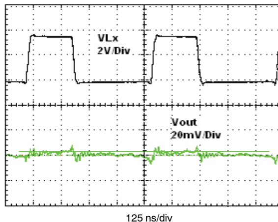
Figure 23. PWM Switching Waveform ( V_{in} = 3.6 \text{ V} , V_{out} = 1.8 \text{ V} , I_{out} = 300 \text{ mA} )
