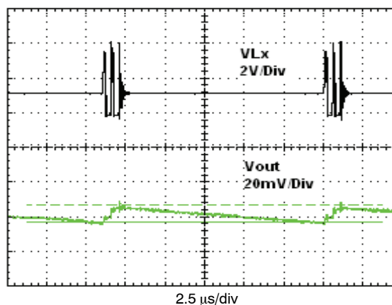
Figure 24. PFM Mode Switching Waveform ( V_{in} = 3.6 \text{ V} , V_{out} = 1.8 \text{ V} , I_{out} = 30 \text{ mA} )
