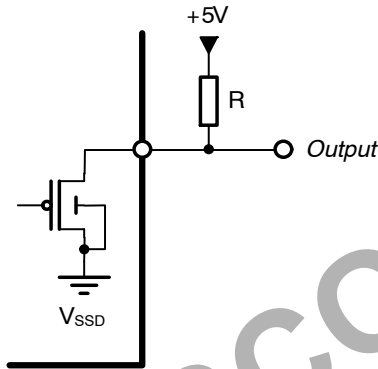
Figure 34. Interfacing to 5 V logic using a 5 V safe output and a pull-up resistor
