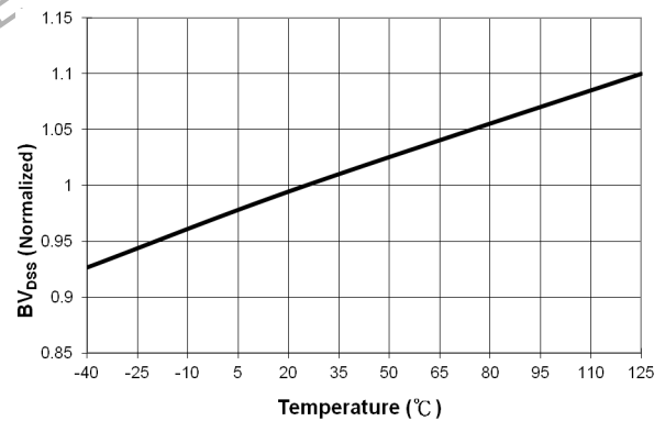
Figure 32. FSL538H/A BV_{DSS} vs. Temperature
