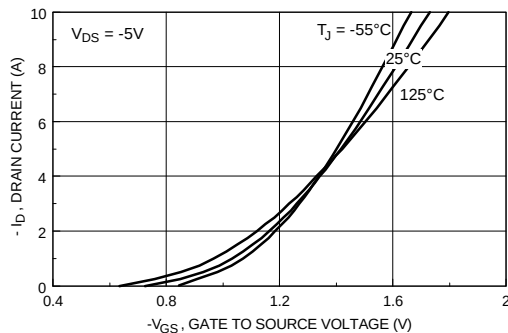
Figure 15. Transfer Characteristics.
