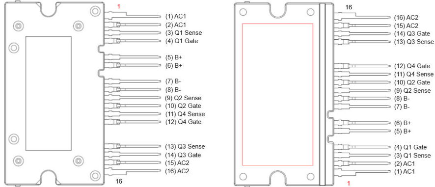
Figure 1. Pin Configuration
